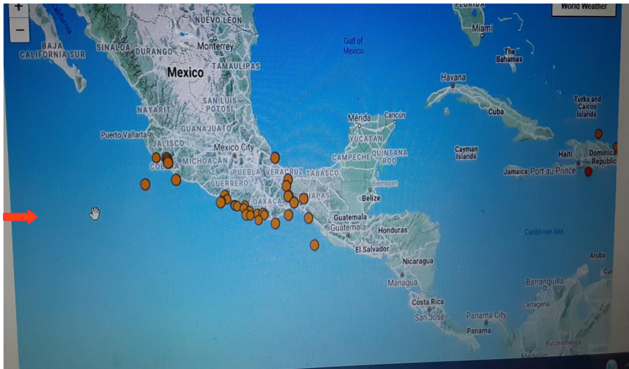
As of March 5, 2021-Central America-Swarms of quakes for over a year.
